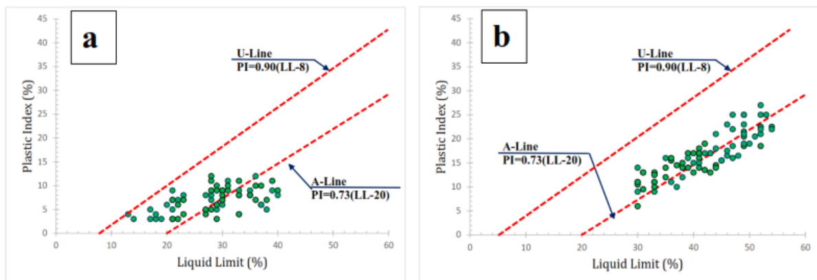
Figure 7. The graph of the changes in the plasticity limit according to the liquid limit of the fine-grained soil of the southern coast of the Caspian Sea: (a) fine-grained soil of the east coast and (b) fine-grained soil of the central-west coast
