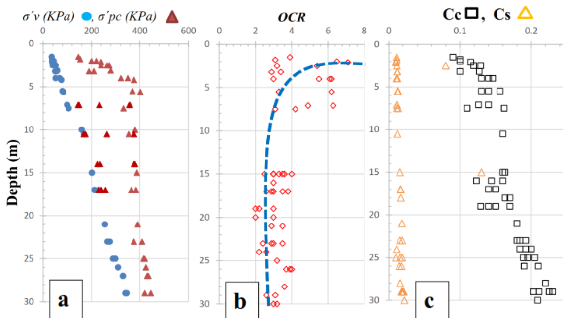
Figure 8. Consolidation of fine-grained soils of the southern coast of the Caspian Sea: (a) effective in situ stress ( \sigma'v ) and maximum experienced stress ( \sigma'pc ) versus depth, (b) overconsolidation ratio (OCR) versus depth, and (c) compression index ( Cc ) and swelling index ( Cs ) versus depth
