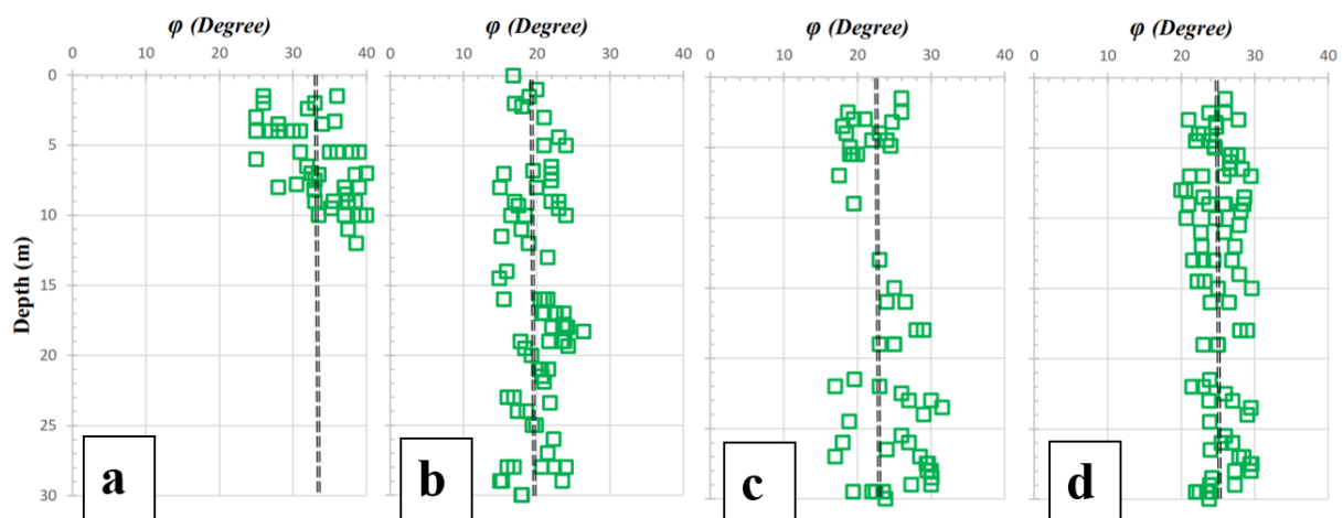
Figure 10. Diagram of the \phi obtained from the direct shear test against depth: (a) Gravel layer, (b) low plasticity Clay layer, (c) Sand layer with fine content, and (d) poorly graded Sand layer
