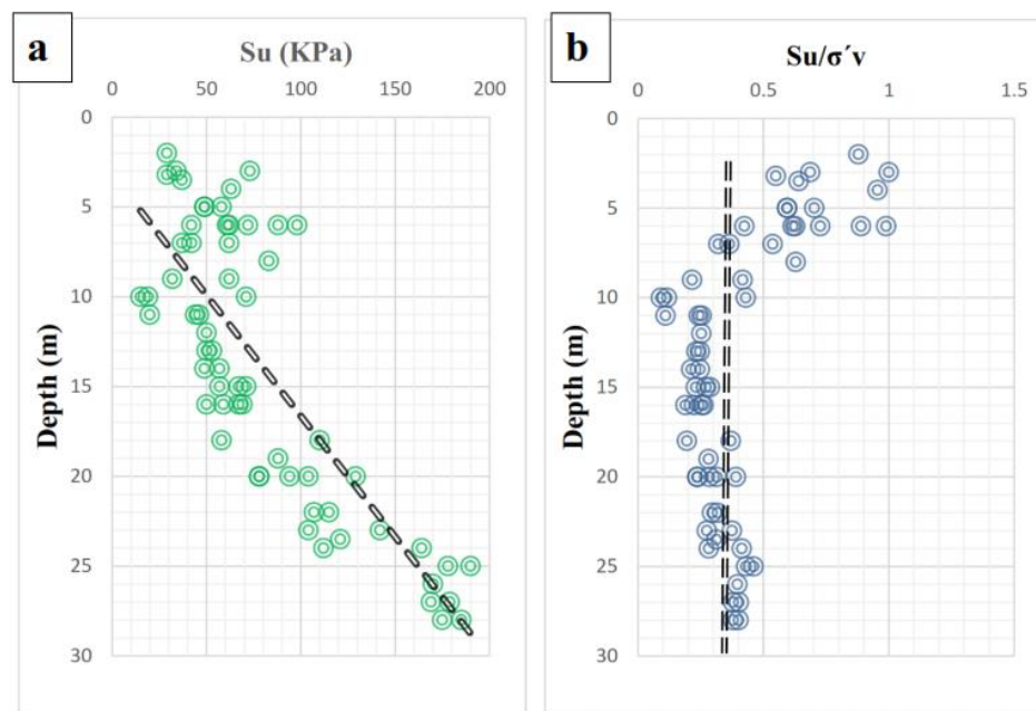
Figure 9. Undrained shear strength ( S_u ) obtained from unconfined compression (UC) test: (a) undrained shear strength versus depth and (b) normalized S_u values versus effective stress versus depth
