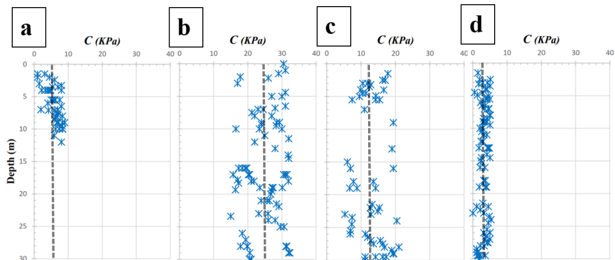
Figure 11. The graph of changes in cohesion values obtained from the direct shear test against depth: (a) Gravel layer, (b) Clay layer with low plasticity, (c) Sand layer with fine content, and (d) poorly graded Sand layer
