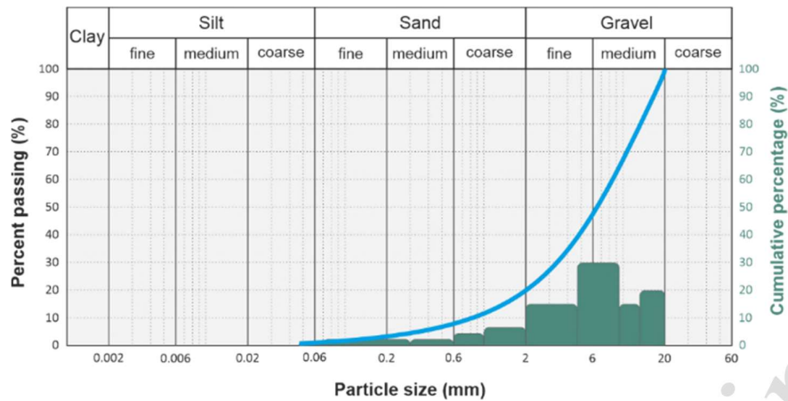
Figure 1. Granulometry curve of the test specimen
