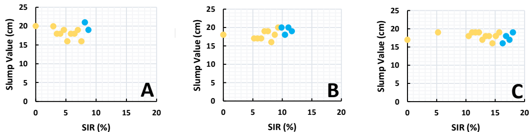
Figure 12. Changes in the slump value after the addition of A: Water, B: Suspension 2.5%, and C: Suspension 5%. ● Dampen loose state, ● Semi uniform non plastic
