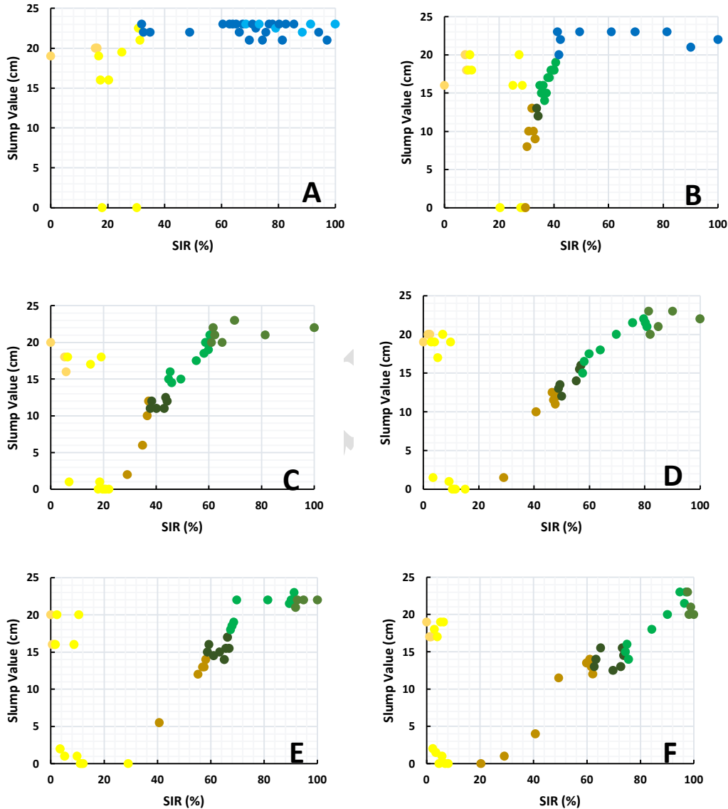
Figure 15. Trend of changes in slump value of the conditioned mix with increasing the injection rate for various suspensions. A: 7.5%, B: 10%, C: 12.5%, D: 15%, E: 17.5%, F: 20%
