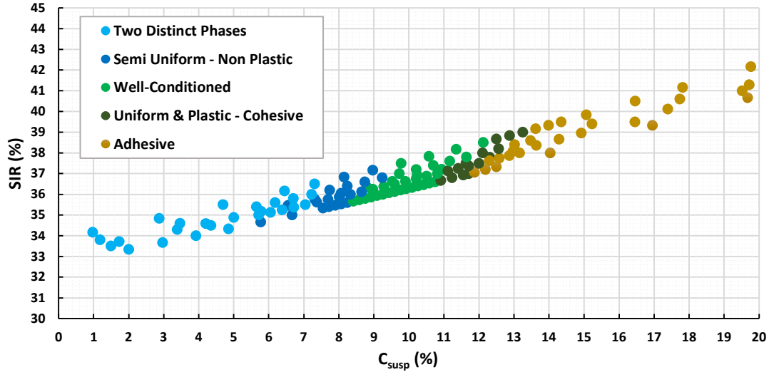
Figure 9. The effect of increasing suspension concentration on the behavior of the conditioned mix
