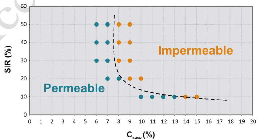
Figure 16. Trend of changes in the state of permeability of the bentonite conditioned material with varying concentrations and injection rates of bentonite suspensions
