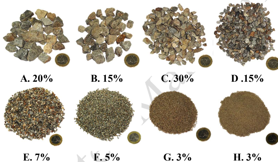
Figure 2. Dominant grain sizes in the test specimen. A: Medium Gravel (19 - 12.5 mm), B: Medium Gravel (12.5 - 9.5 mm), C: Medium-Fine Gravel (9.5 - 4.75 mm), D: Fine Gravel (4.75 - 2.00 mm), E: Coarse Sand (2.00 - 1.18 mm), F: Coarse Sand (1.18 - 0.59 mm), G: Medium Sand (0.59 - 0.29 mm), H: Medium-Fine Sand (0.29 - 0.074 mm)
