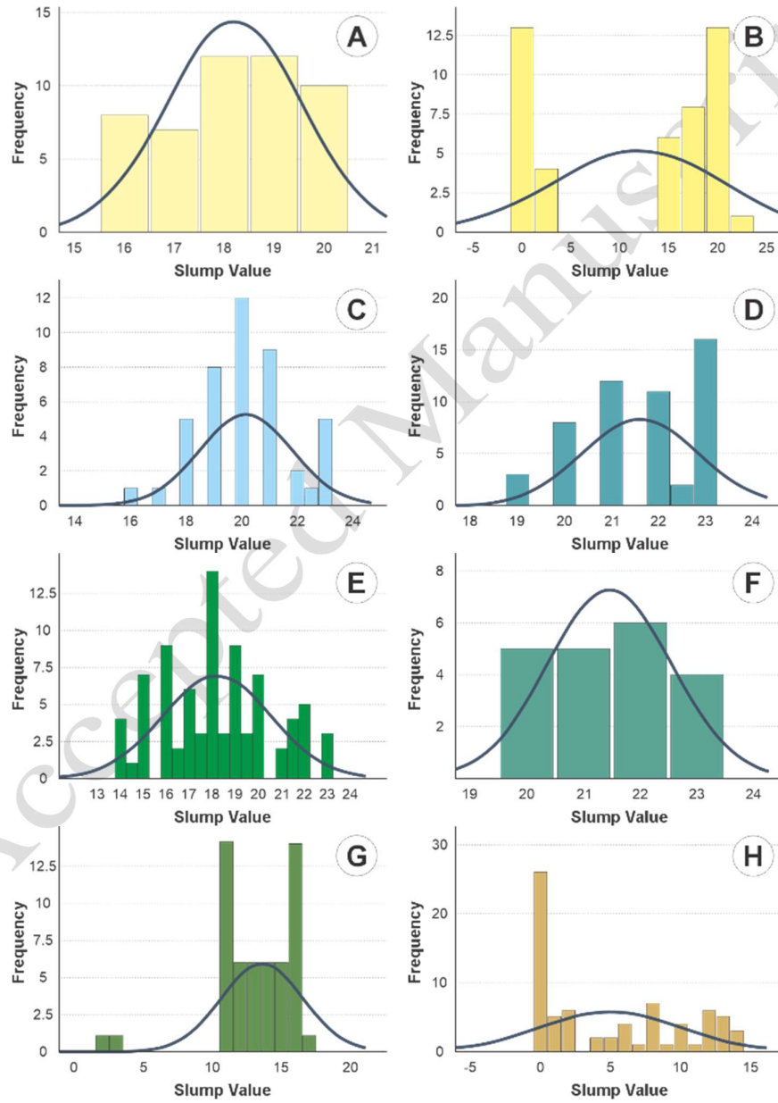
Figure 19. Frequency of the slump values for all different states of conditioned material's behavior. A: Dampened Loose, B: Unstable Low slump, C: Distinct Phases, D: Semi Uniform non-Plastic, E: Well-Conditioned, F: Over Conditioned, G: Cohesive, H: Adhesive
