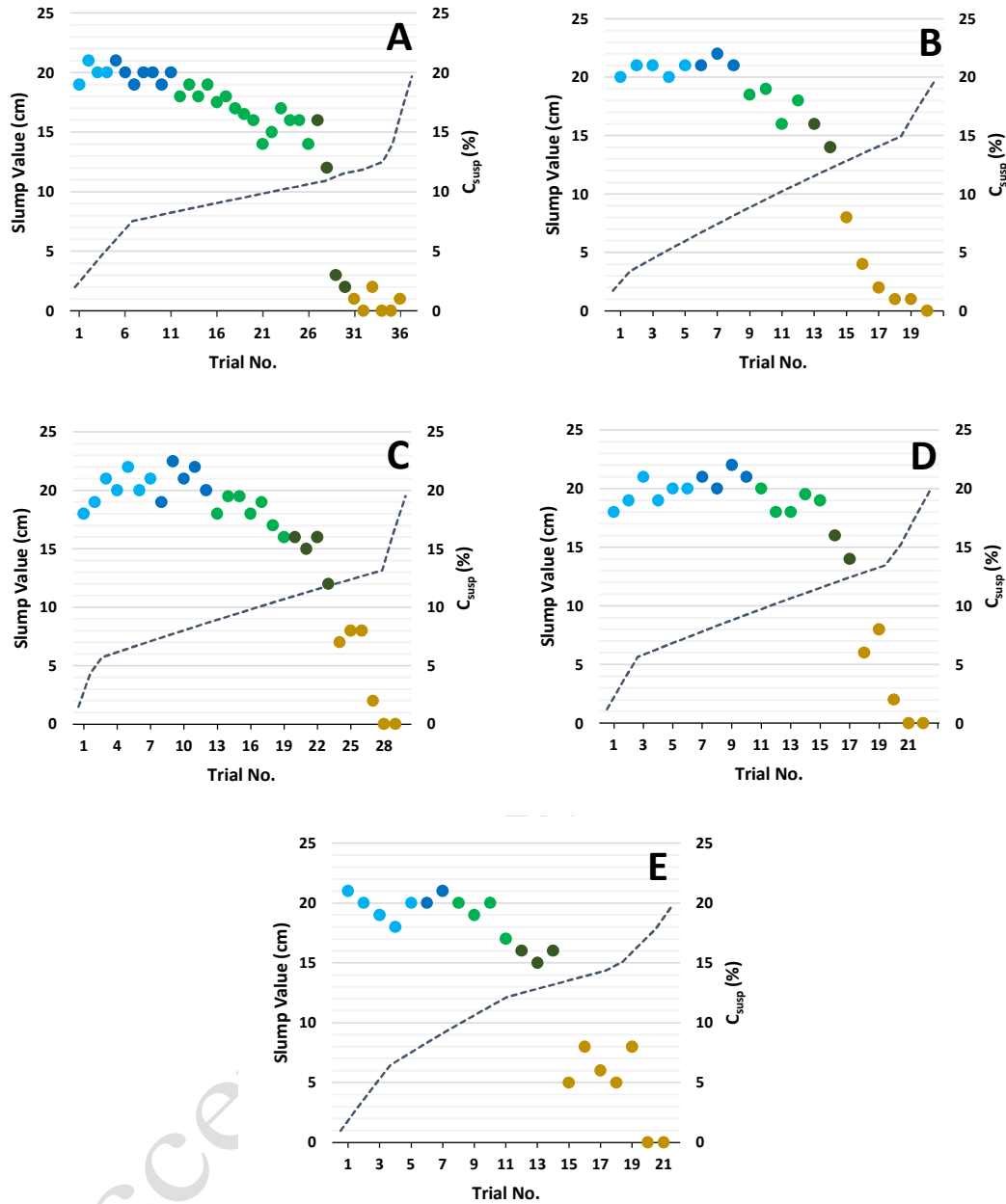
Figure 3. Slump values of test specimens after the addition of dry bentonite and trend of changes in the created suspension concentration ( C_{susp} ) in the mix. A: 15Kg Specimen, B: 17.2Kg Specimen, C: 20Kg Specimen, D: 25Kg Specimen, E: 30Kg Specimen
