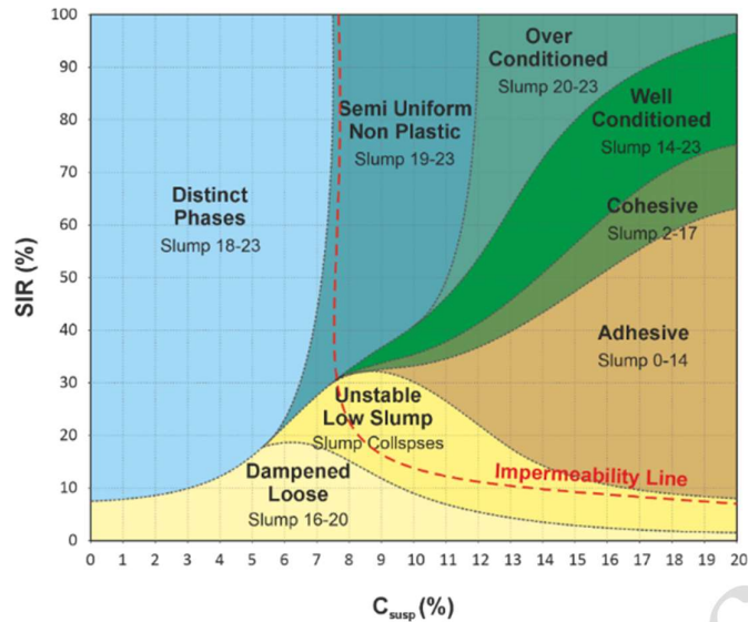
Figure 20. Empirical model illustrating the different states of behavior exhibited by Bentonite conditioned excavated material
