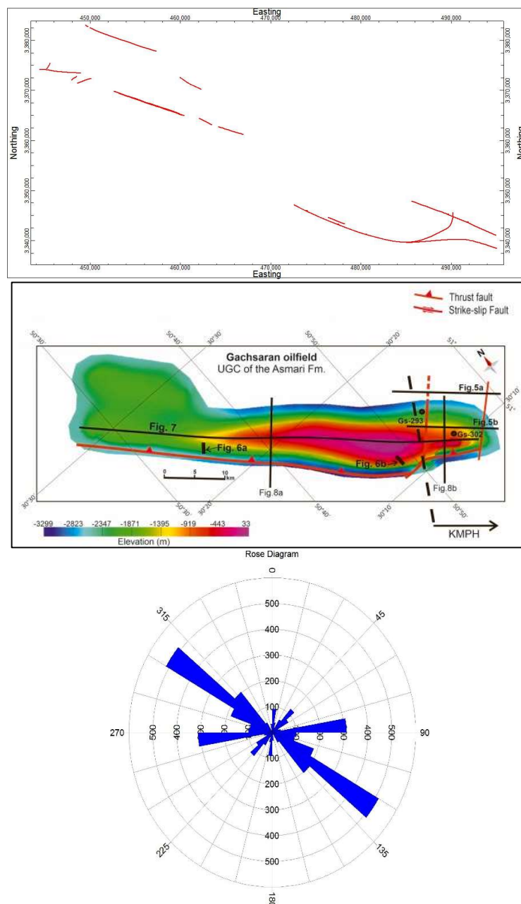
Figure 2. Fault map (based on Shamszadeh et al., 2022) and rose diagram of the Gachsaran oilfield
