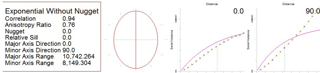
Figure 4. Variogram and anisotropic ellipsoid for effective porosity
