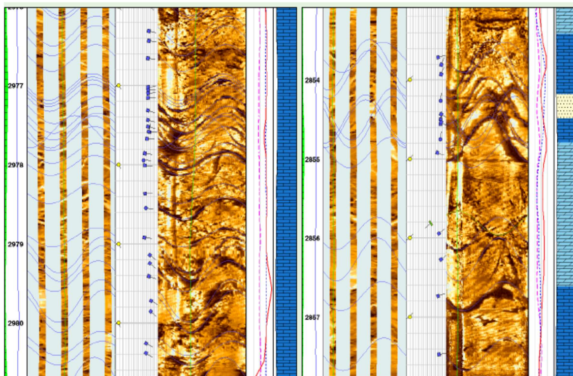
Figure 10. Open fractures in the Asmari reservoir of the Gachsaran oilfield in two image logs
