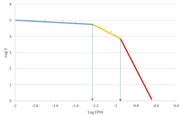
Figure 6. The C-V log-log plot of effective porosity and related threshold values
