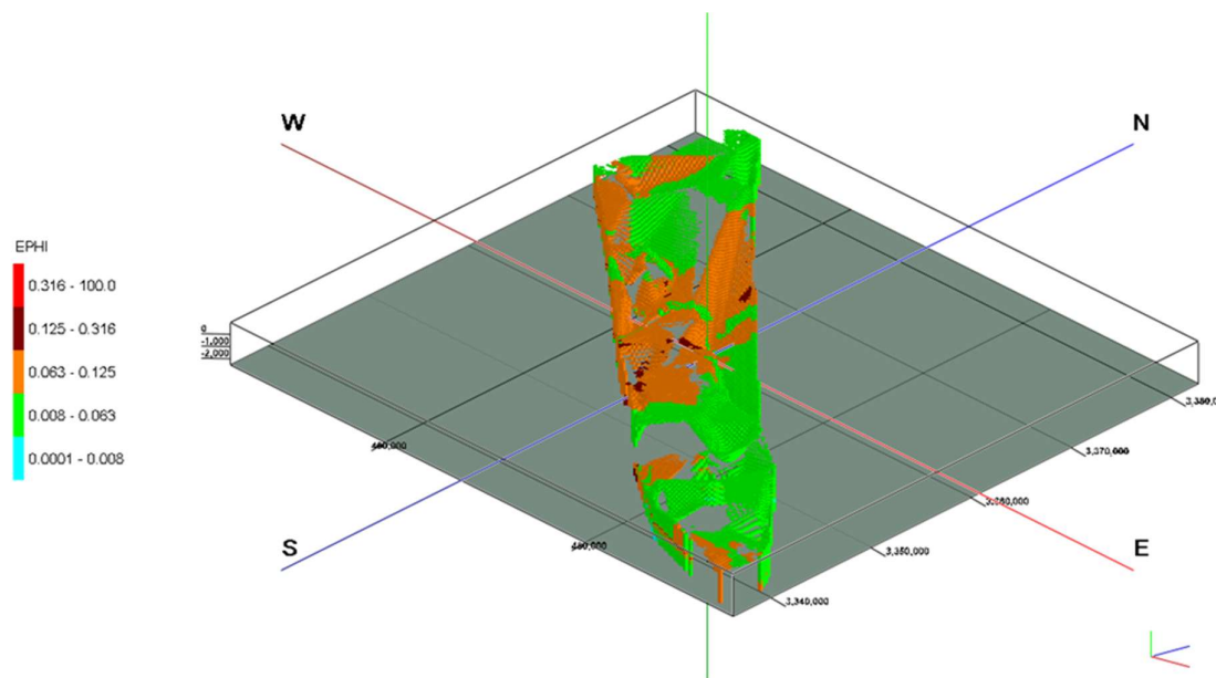
Figure 9. Effective porosity zones' distribution map of the effective porosity obtained by the N-S method in the study oilfield
