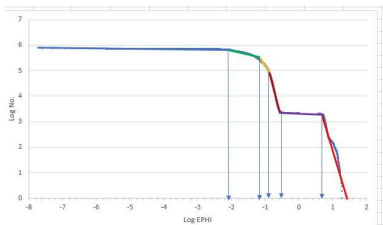
Figure 8. The N-S log-log of effective porosity
