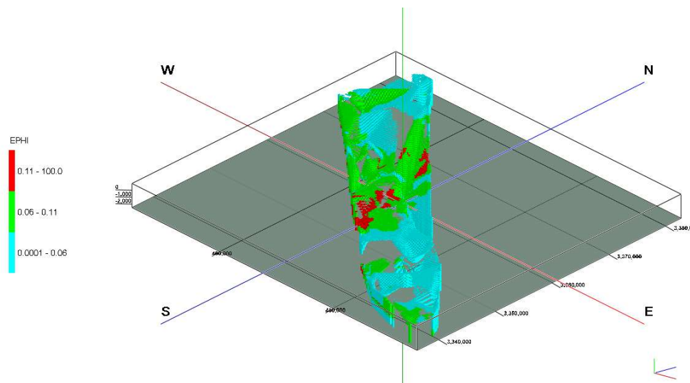
Figure 7. Effective porosity zones' distribution map of the effective porosity via the C-V model in the study oilfield
