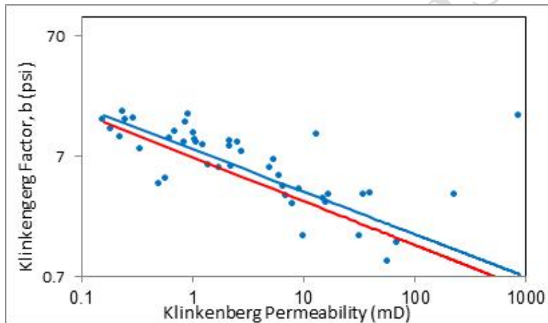
Figure 6. Klinkenberg factor, b versus Klinkenberg permeability of selected samples (blue points) and in comparison with Jones, 1972 model (red line)
