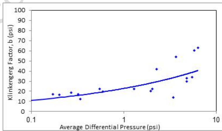
Figure 11. Klinkenberg factor, b (psi) versus average differential pressure (psi) by constant backpressure test for selected samples
