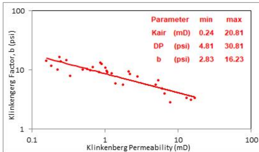
Figure 12. Klinkenberg factor, b (psi) versus Klinkenberg permeability (mD) by constant mass flow rate method for selected samples
