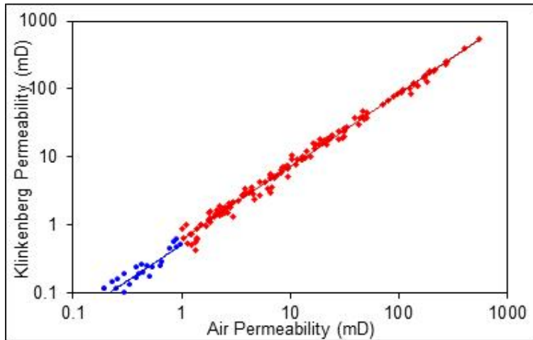
Figure 5. laboratory Klinkenberg permeability data measured versus air permeability. In the low permeability range (less than 1 mD), the decrease in Klinkenberg permeability is greater than in the higher permeability range
