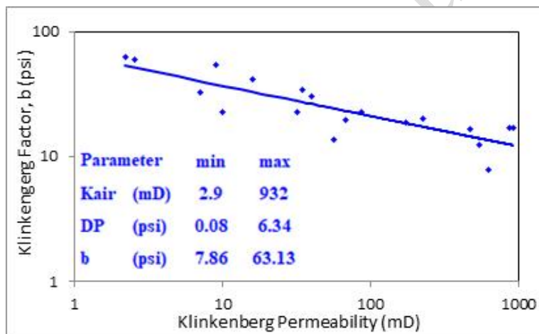
Figure 10. Klinkenberg factor, b (psi) versus Klinkenberg permeability (mD) by constant backpressure test for selected samples
