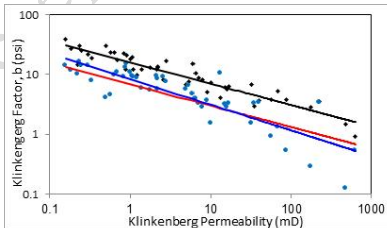
Figure 7. Klinkenberg factor, b (psi) versus Klinkenberg permeability (mD) by Helium gas (black points) and Nitrogen gas (blue points) injection in selected samples and comparison with Jones 1972 model (red line), for selected samples.
