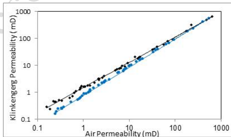
Figure 8. Klinkenberg permeability ( K_L ) versus Air Permeability by steady-state (blue points) and unsteady-state (black points) methods for selected samples
