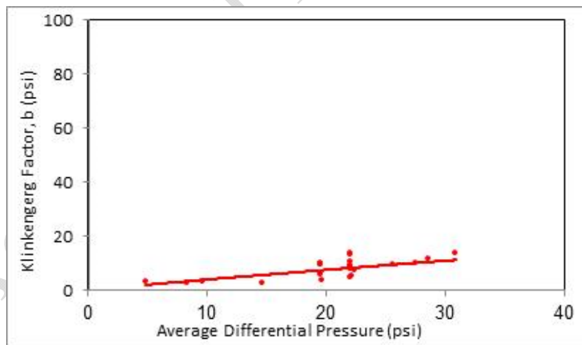
Figure 13. Klinkenberg factor, b (psi) versus average differential pressure (psi) by constant mass flow rate method for selected samples
