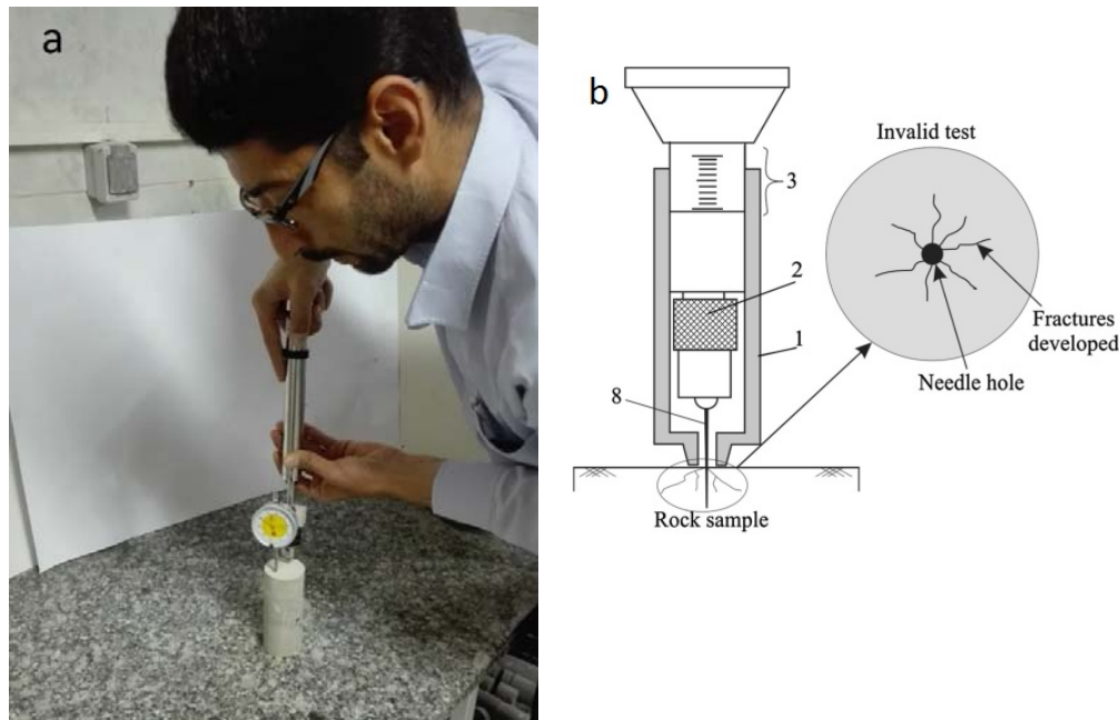
Figure 3. a: Application of the needle penetrometer in laboratory on core, b: Schematic illustration of an invalid NP test (Ulusay & Erguler, 2012).
