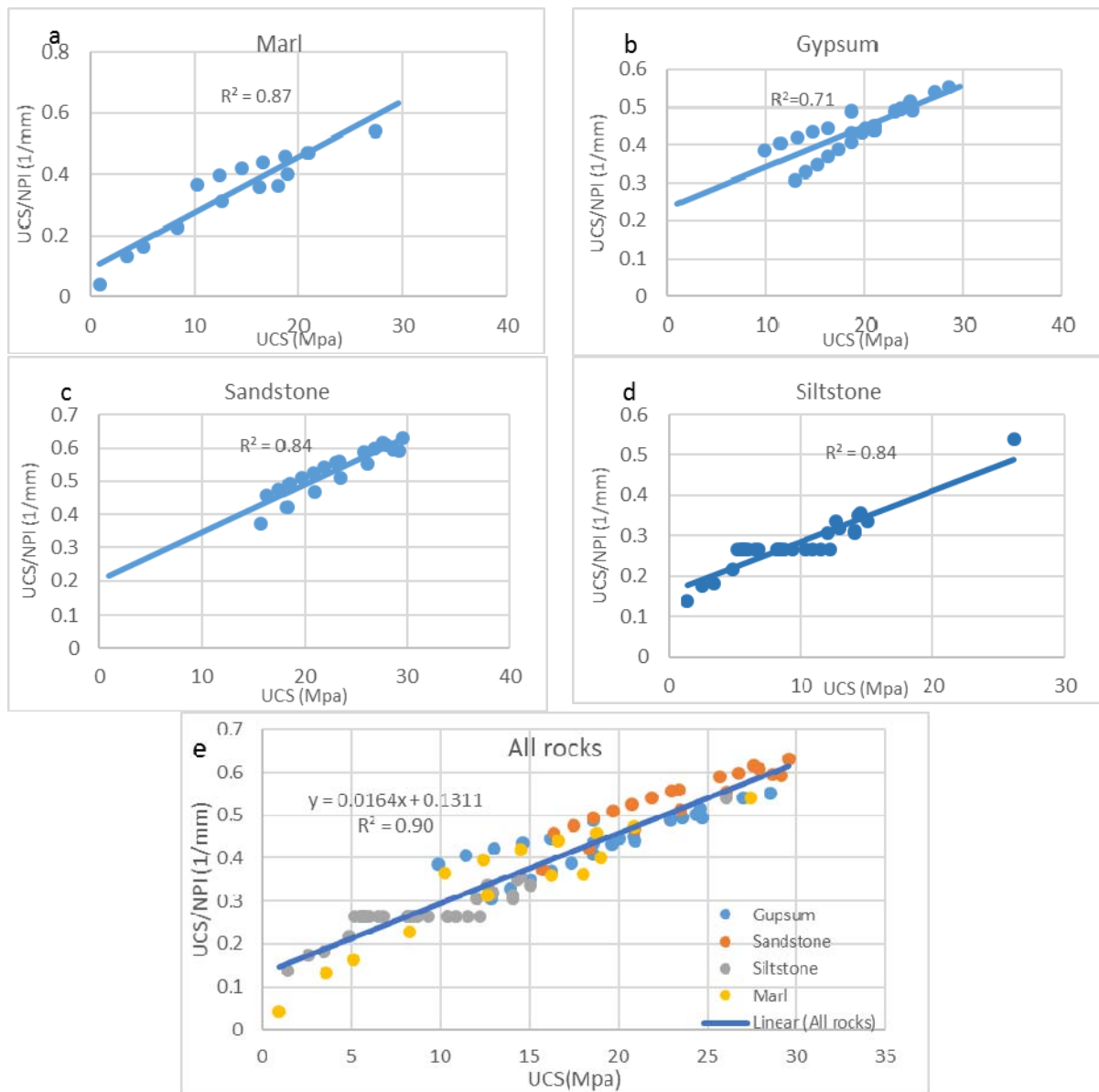
Figure 6. Relationship between the ratio of UCS/NPI and the UCS of intact rocks for a) Marl, b) Gypsum, c) Sandstone, d) Siltstone and e) all rock types.
