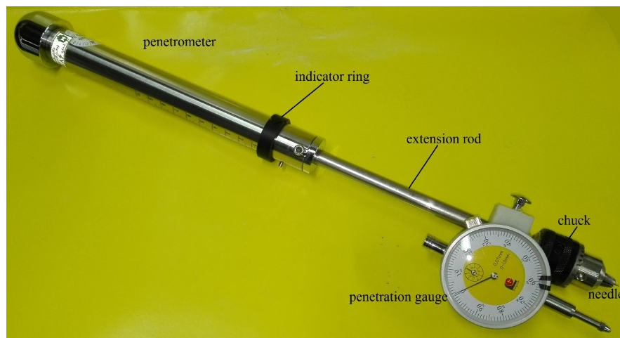
Figure 2. Modified Eijkelkamp Needle penetrometer device.
