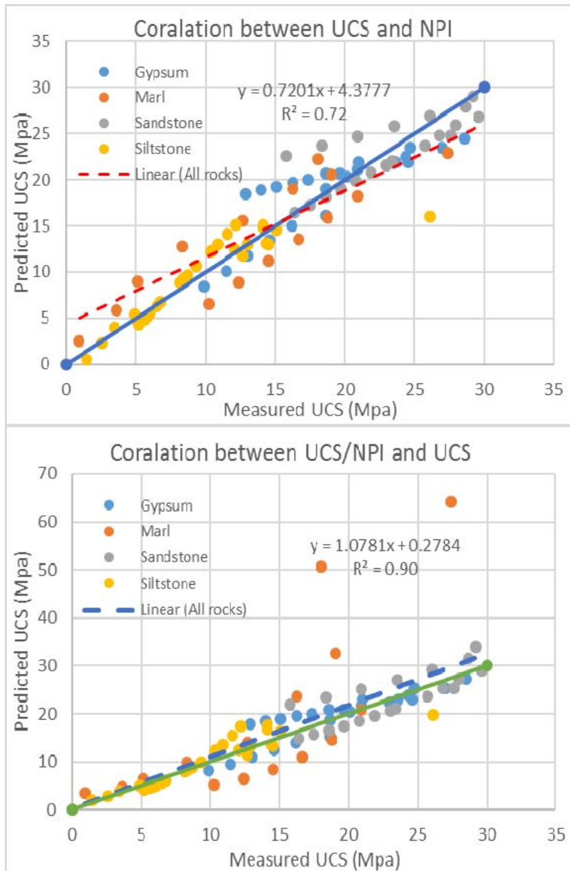
Figure 7. Comparison between the measured and the computed UCS from a) NPI vs. UCS plot and b) UCS/NPI vs. UCS plot.
