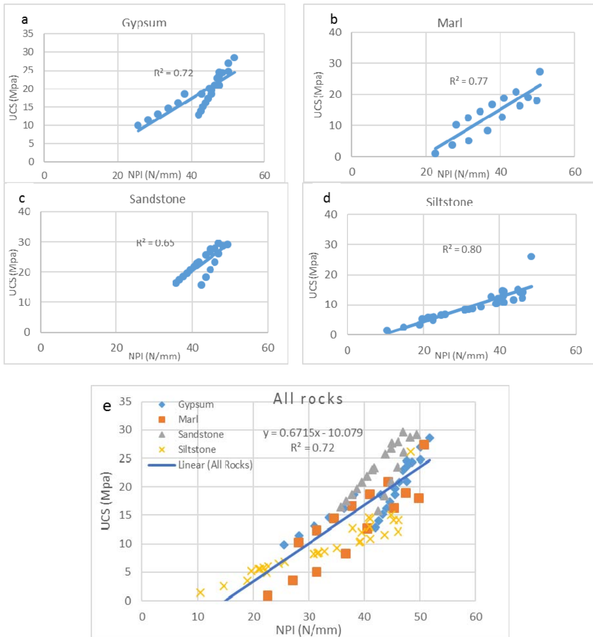
Figure 5. Simple regression analyses between the NPI and the UCS for a: Gypsum, b: Marl, c: Sandstone, d: Siltstone and e: all rock types.
