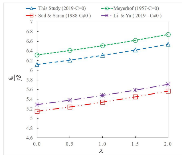
Figure 9. Comparison of the present study with other researchers in different positions of the foundation from edge of slope relative to its width ( \lambda ) in the inclined land on cohesive and non-cohesive soils in for: \phi = 40^\circ , \beta = 45^\circ , B = 2
