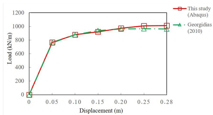
Figure 4. Comparison of vertical load-settlement changes for \theta=0 in this study and Georgiadis (2010)
