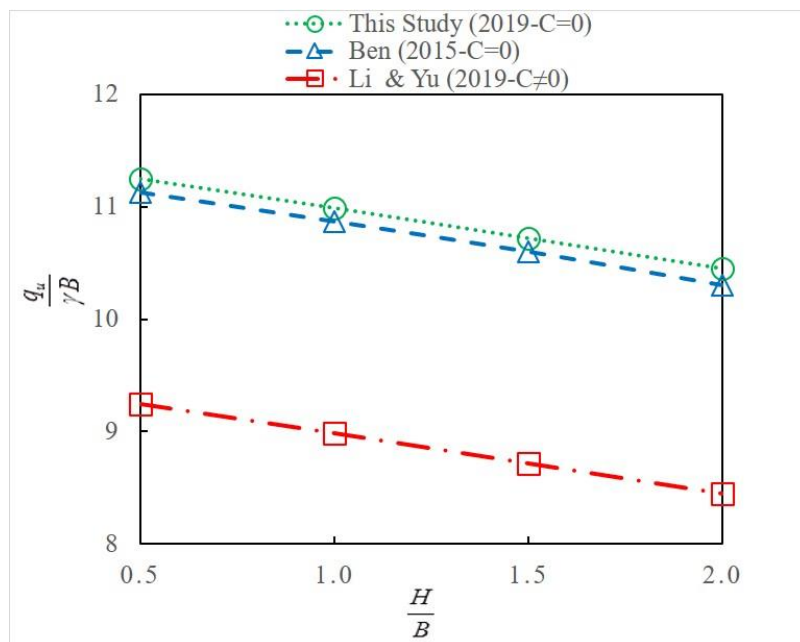
Figure 12. Comparison of the present study with other researchers in different positions of the height of slope relative to the foundation width ( \frac{H}{B} ) in the inclined land on cohesive and non-cohesive soils in for: \phi = 40^\circ , \beta = 45^\circ , B = 2
