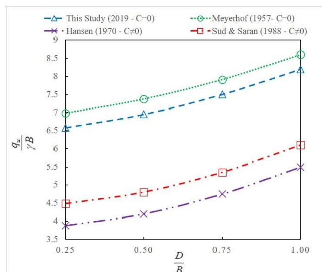
Figure 10. Comparison of the present study with other researchers in different positions of embedded Depth relative to the width of foundation ( \frac{D}{B} ) in the inclined land on cohesive and non-cohesive soils in for: \phi = 40^\circ , \beta = 45^\circ , B = 2
