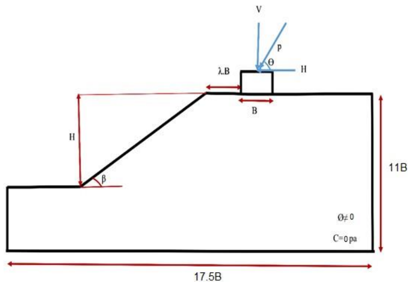
Figure 3. Schematic geometry of the foundation and the type studied in this study
