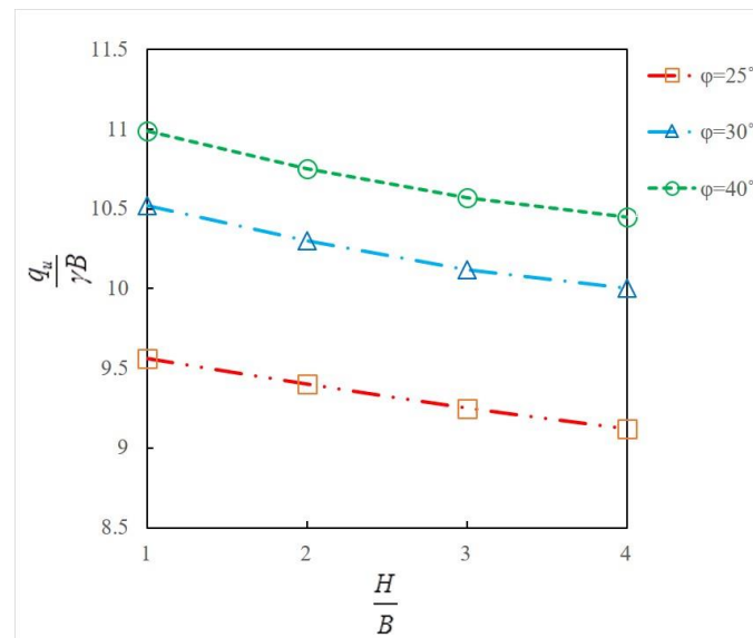
Figure 8. Changes in normalized bearing capacity to relative the height of slope to the width of foundation ( \frac{H}{B} ) for: \lambda = 0 , D \neq 0 , B = 2
