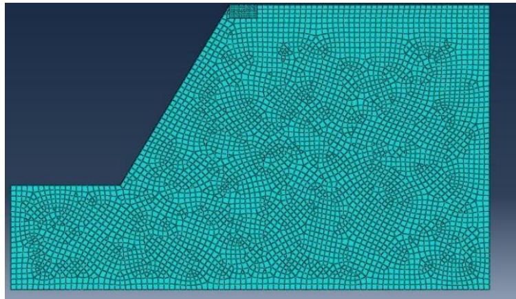
Figure 2. Mesh of general modeling in this study
