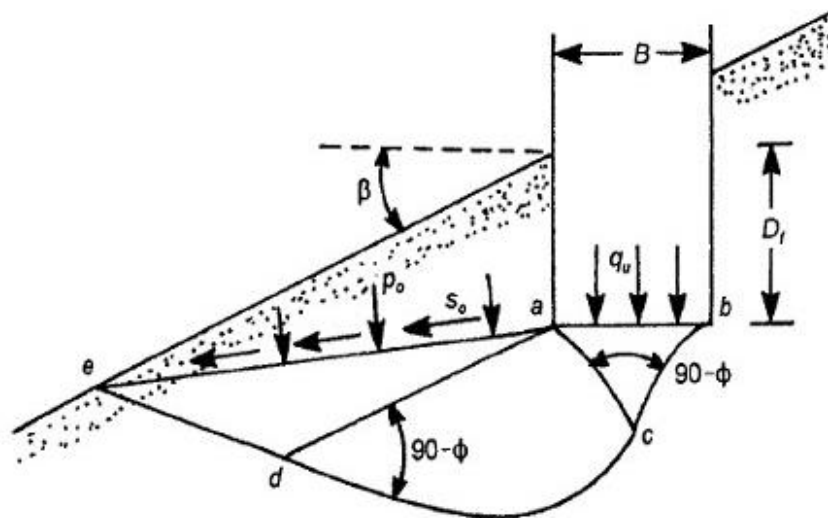
Figure 1. The failure region created under the foundation according to Meyerhof's method (1975)
