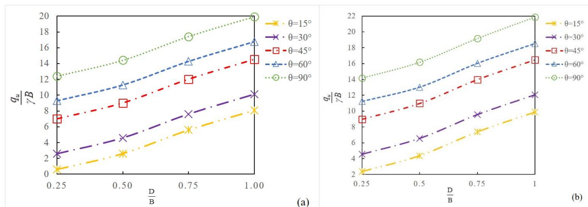
Figure 6. Changes in normalized bearing capacity to load angle ( \theta ) and ratio of embedded Depth to width of foundation ( \frac{D}{B} ) for (a): \phi = 30^\circ , \beta = 45^\circ , B = 2 and (b): \phi = 40^\circ , \beta = 15^\circ , B = 2
