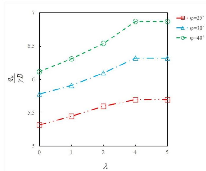
Figure 7. Changes in normalized bearing capacity to relative the distance of the foundation from the slope to the width of the foundation ( \lambda ) for: \lambda \neq 0 , \beta = 45^\circ , B = 2
