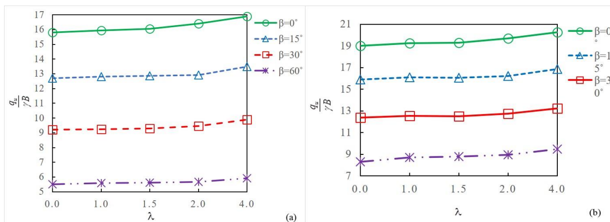
Figure 5. Changes in the normalized bearing capacity to the slope angle ( \beta ) and the ratio of the distance of foundation from edge of slope to the its width ( \lambda ) for (a): \phi = 30^\circ , \theta = 45^\circ , B = 2 and (b): \phi = 40^\circ , \theta = 60^\circ , B = 2
