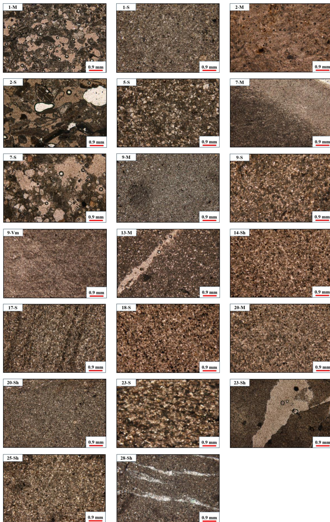
Figure 3. Microscopic images of lithological thin sections
