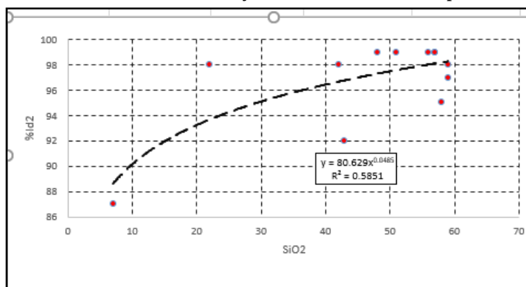
Figure 12. Correlation of durability index and SiO 2 percentage
